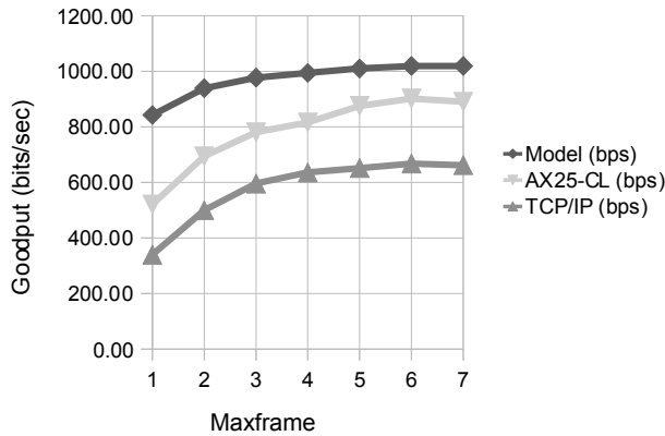
Fig. 4. Comparison of transfer times for AX.25CM-CL and TCP/AX.25 with reference to theoretical model at 1200bps.
