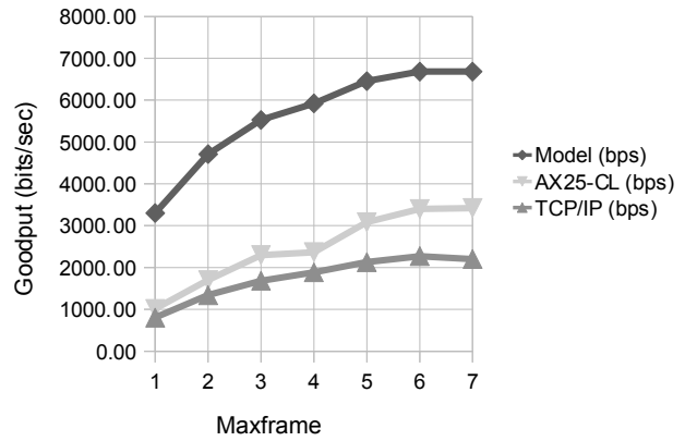
Fig. 5. Comparison of transfer times for AX.25CM-CL and TCP/AX.25 with reference to theoretical model at 9600bps
